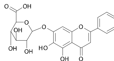
Baicalin
