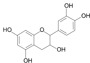
Catechin
